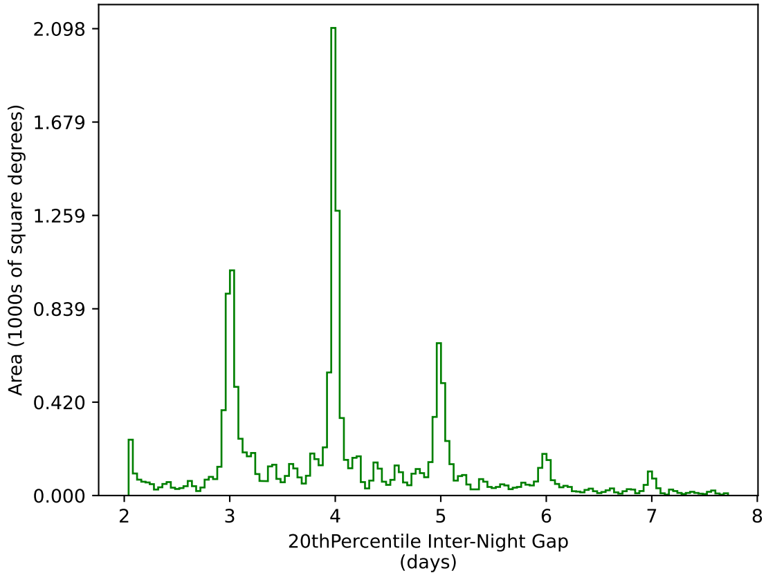
too_elab_r8_d2_ugrizy_v3.4_10yrs WFD g band: 20thPercentile Inter-Night Gap
