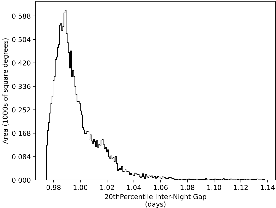
too_elab_r8_d2_ugrizy_v3.4_10yrs WFD all bands: 20thPercentile Inter-Night Gap
