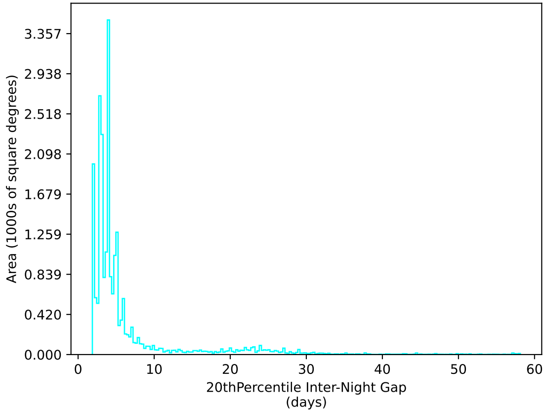
too_elab_r8_d2_ugrizy_v3.4_10yrs All sky u band: 20thPercentile Inter-Night Gap
