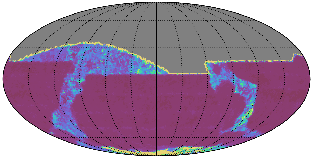
too_elab_r8_d2_ugrizy_v3.4_10yrs All sky r band: 20thPercentile Inter-Night Gap
