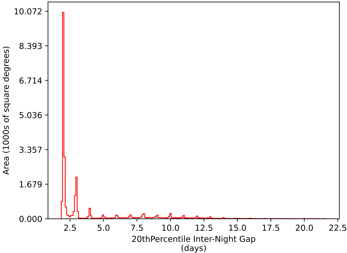
too_elab_r8_d2_ugrizy_v3.4_10yrs All sky i band: 20thPercentile Inter-Night Gap
