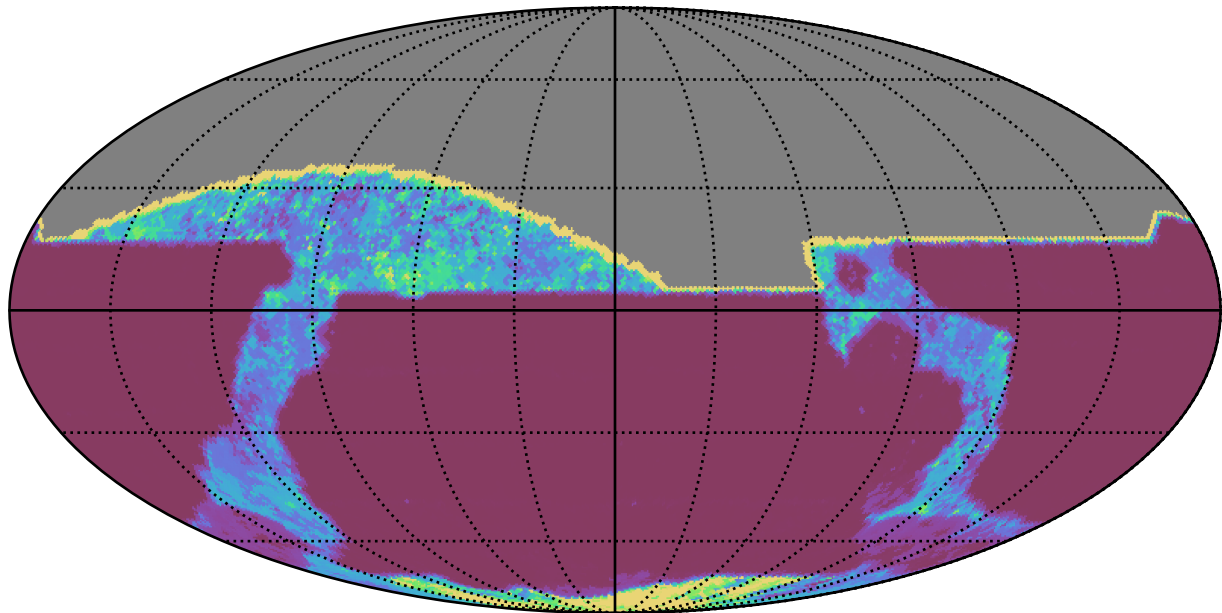
too_elab_r8_d2_ugrizy_v3.4_10yrs All sky all bands: 20thPercentile Inter-Night Gap
