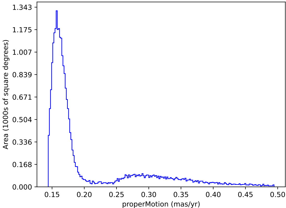
too_elab_r8_d2_ugrizy_v3.4_10yrs : properMotion
