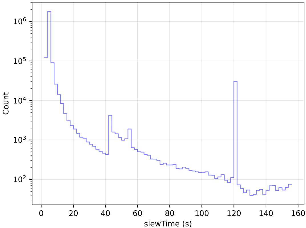
too_elab_r8_d2_ugrizy_v3.4_10yrs All visits: Slew Time Histogram
