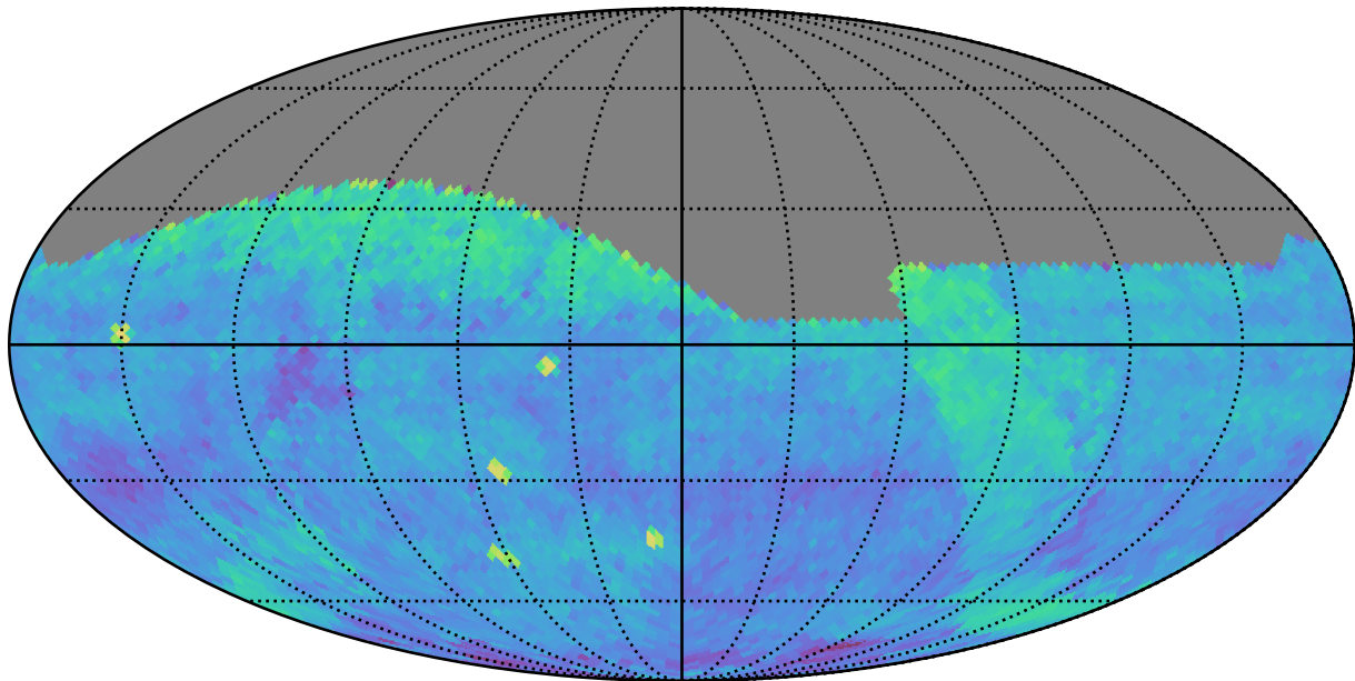
too_elab_r8_d2_ugrizy_v3.4_10yrs (g or r or i): PairFraction
