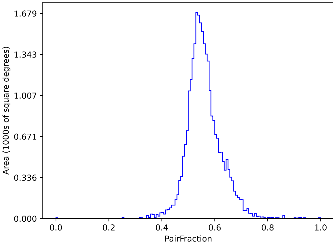
too_elab_r8_d2_ugrizy_v3.4_10yrs (g or r or i): PairFraction
