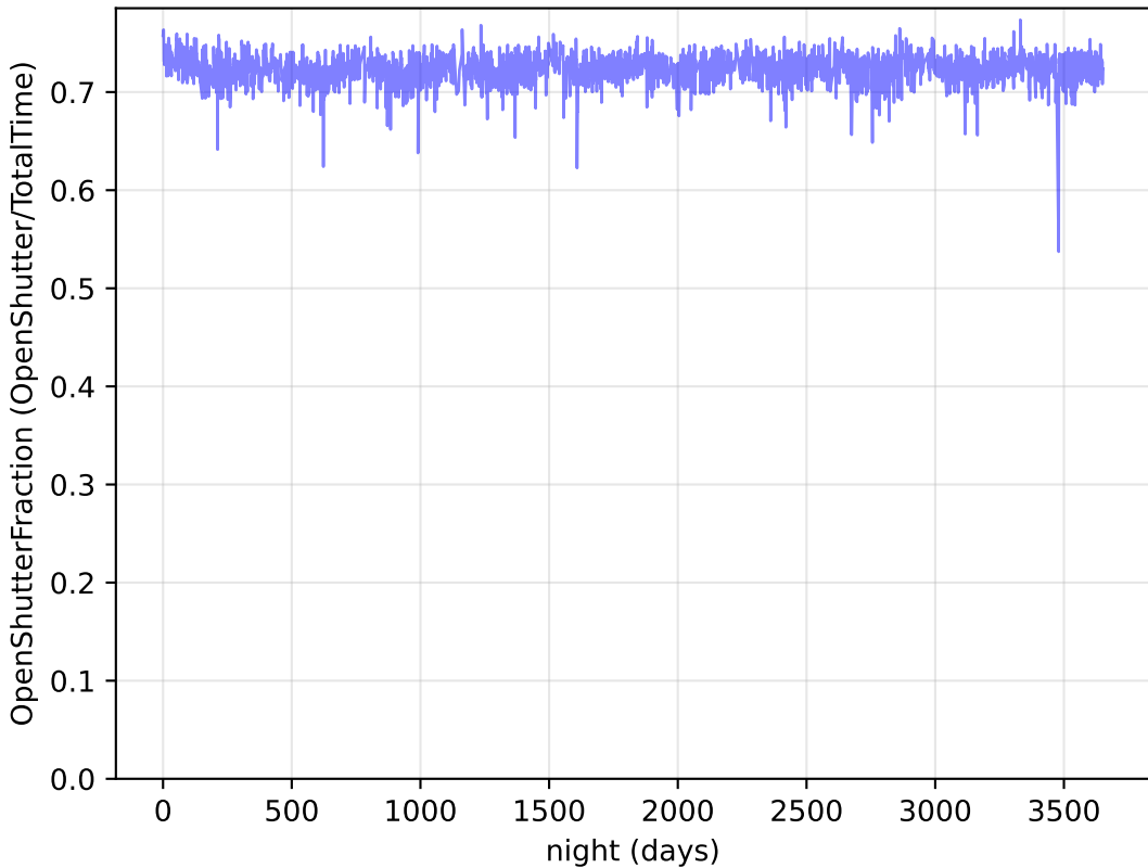
too_elab_r8_d2_ugrizy_v3.4_10yrs : OpenShutterFraction
