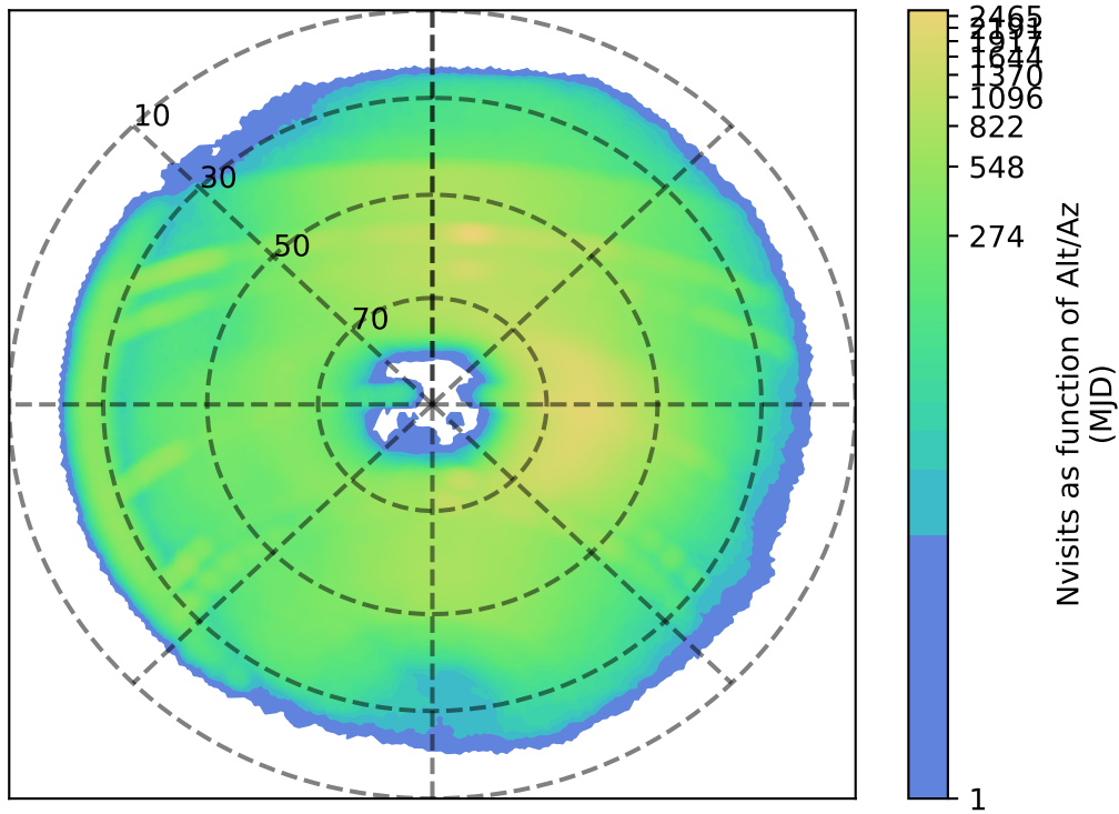
too_elab_r8_d2_ugrizy_v3.4_10yrs r: Nvisits as function of Alt/Az
