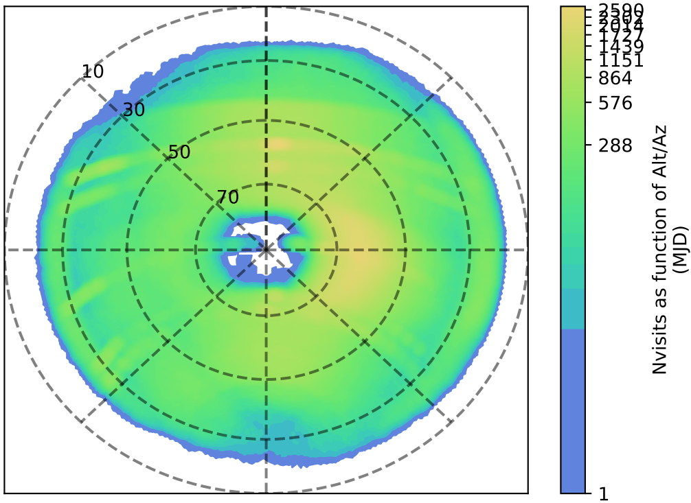
too_elab_r8_d2_ugrizy_v3.4_10yrs i: Nvisits as function of Alt/Az
