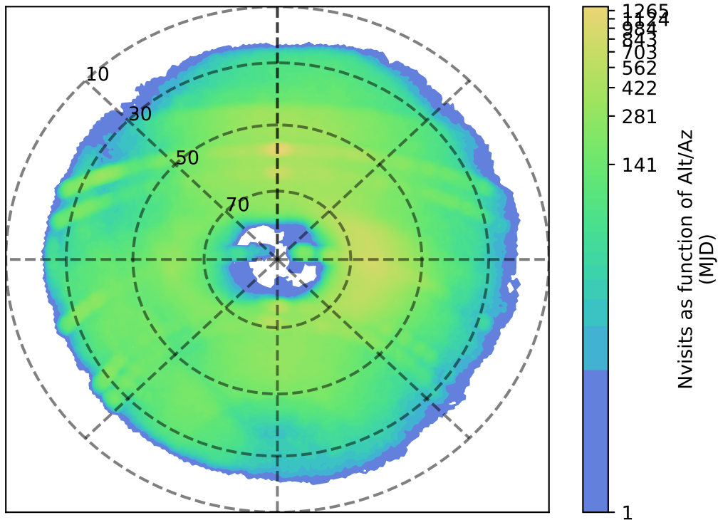
too_elab_r8_d2_ugrizy_v3.4_10yrs g: Nvisits as function of Alt/Az
