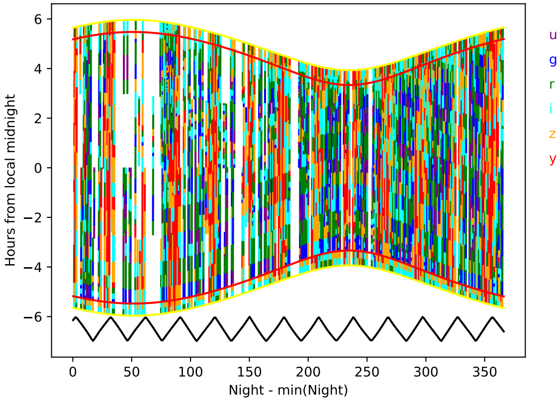
too_elab_r8_d2_ugrizy_v3.4_10yrs year 9-10: Hourglass
