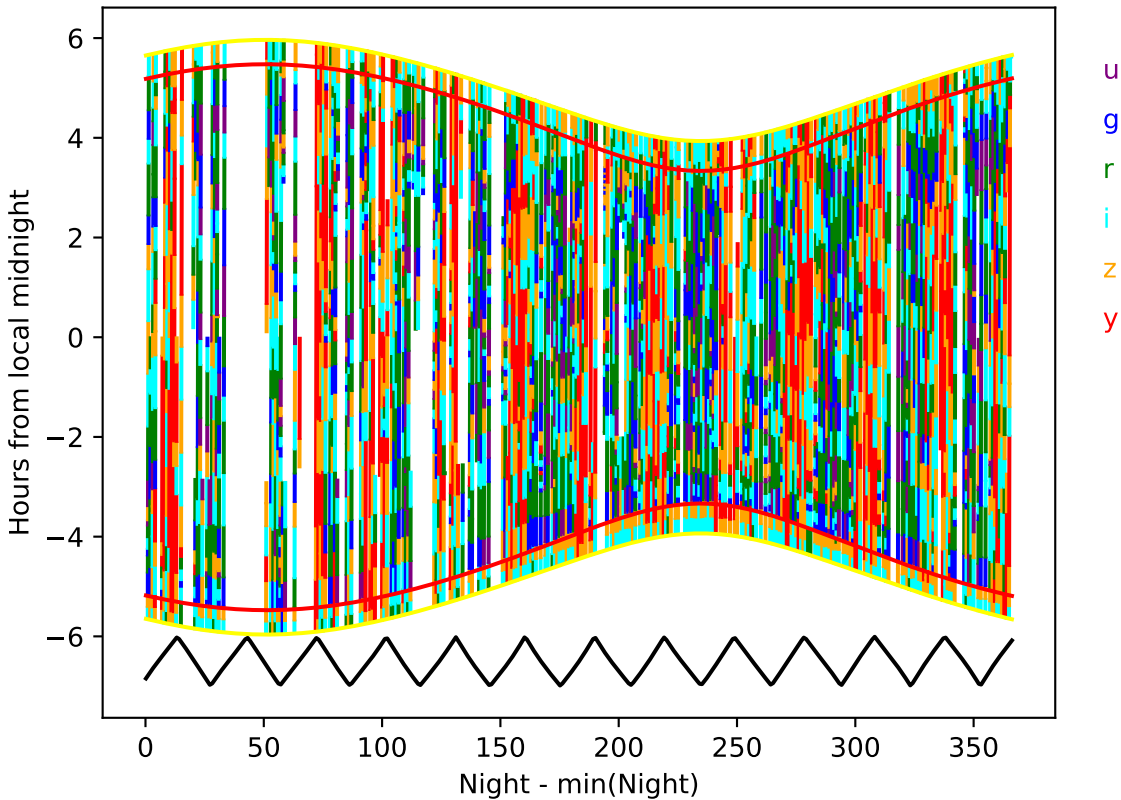
too_elab_r8_d2_ugrizy_v3.4_10yrs year 8-9: Hourglass
