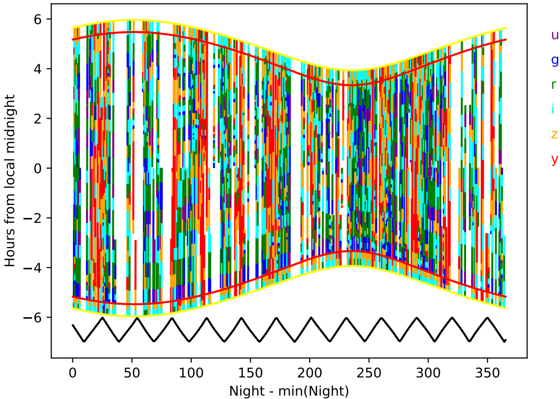
too_elab_r8_d2_ugrizy_v3.4_10yrs year 7-8: Hourglass
