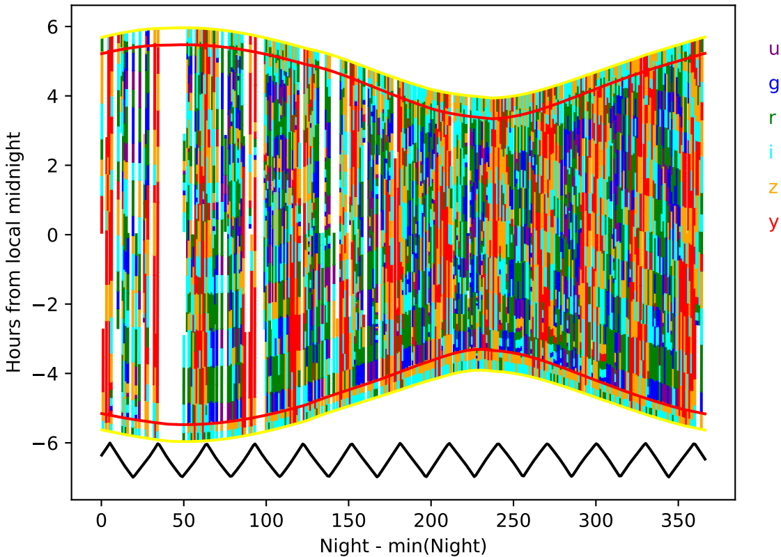
too_elab_r8_d2_ugrizy_v3.4_10yrs year 6-7: Hourglass
