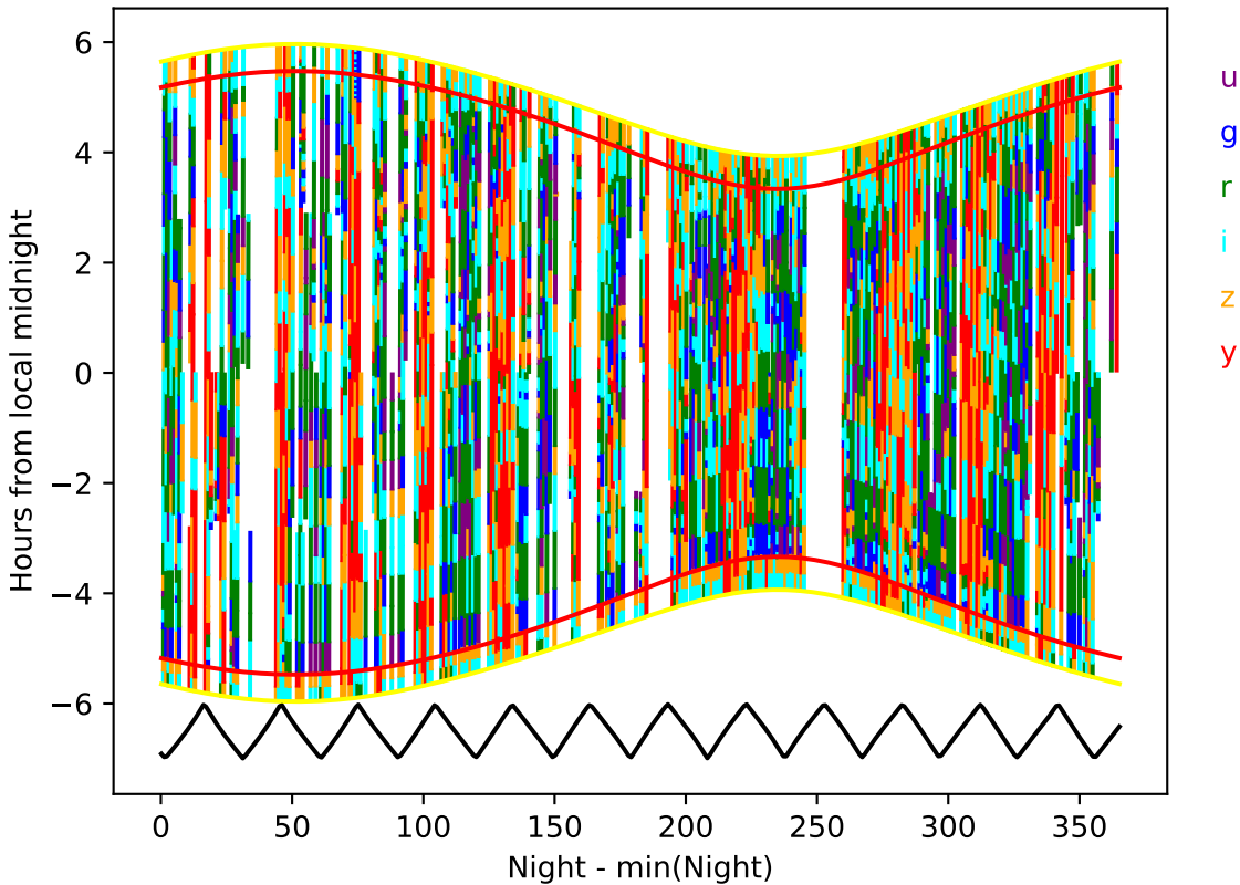
too_elab_r8_d2_ugrizy_v3.4_10yrs year 5-6: Hourglass
