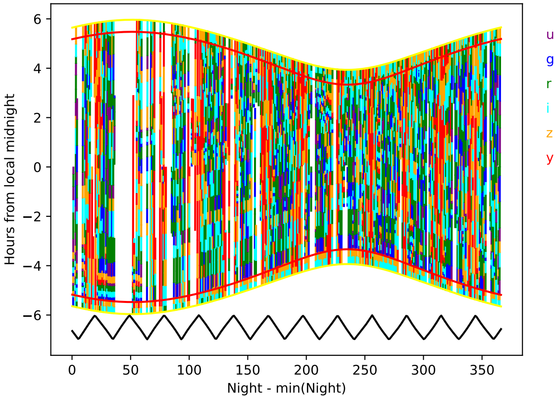
too_elab_r8_d2_ugrizy_v3.4_10yrs year 2-3: Hourglass
