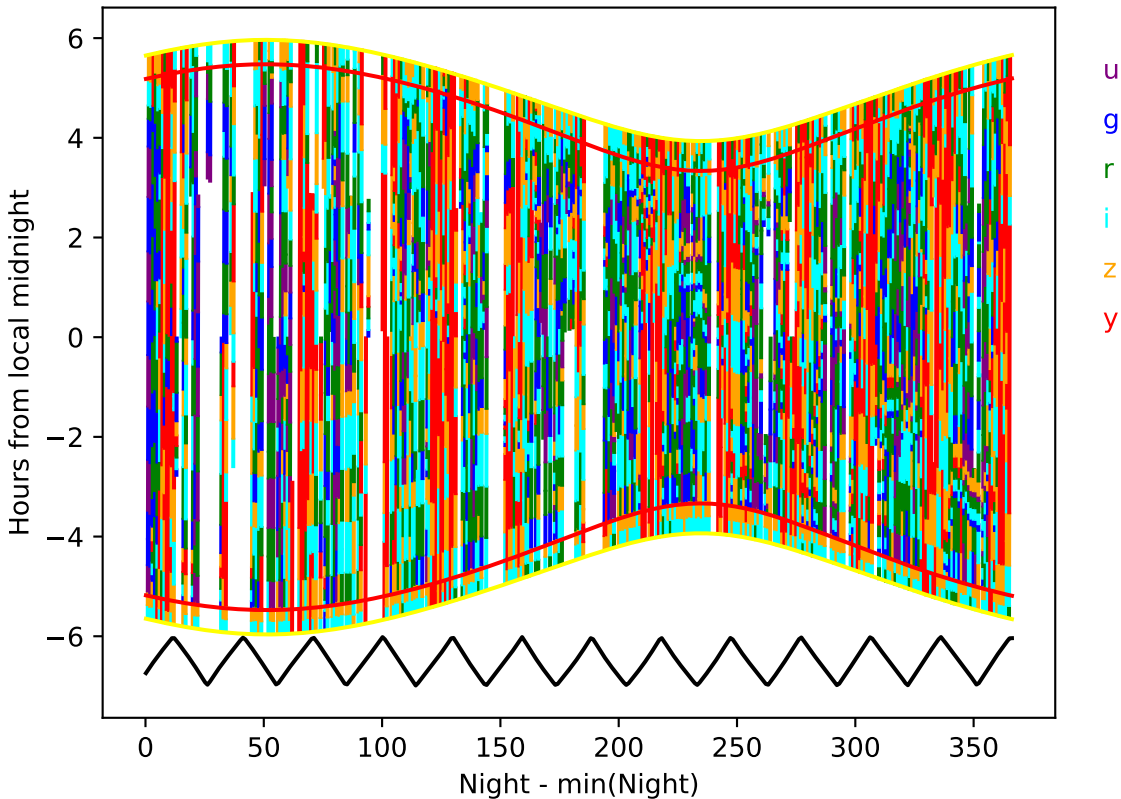
too_elab_r8_d2_ugrizy_v3.4_10yrs year 0-1: Hourglass
