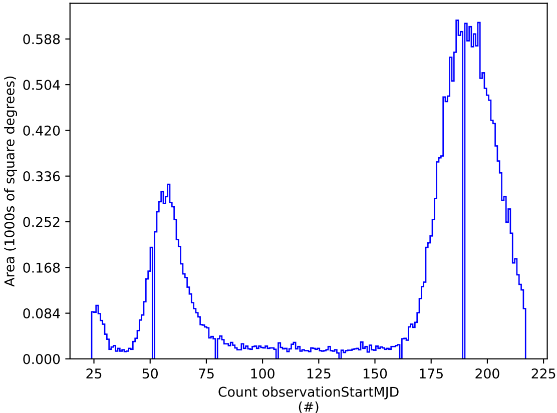
too_elab_r8_d2_ugrizy_v3.4_10yrs i: Count observationStartMJD
