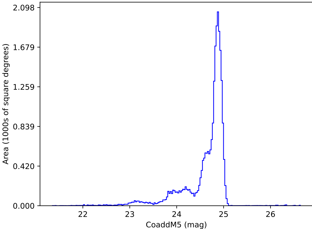
too_elab_r8_d2_ugrizy_v3.4_10yrs y: CoaddM5
