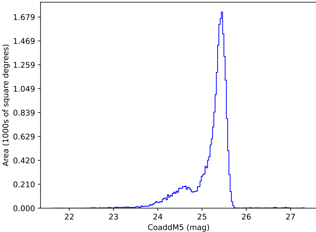
too_elab_r8_d2_ugrizy_v3.4_10yrs u: CoaddM5
