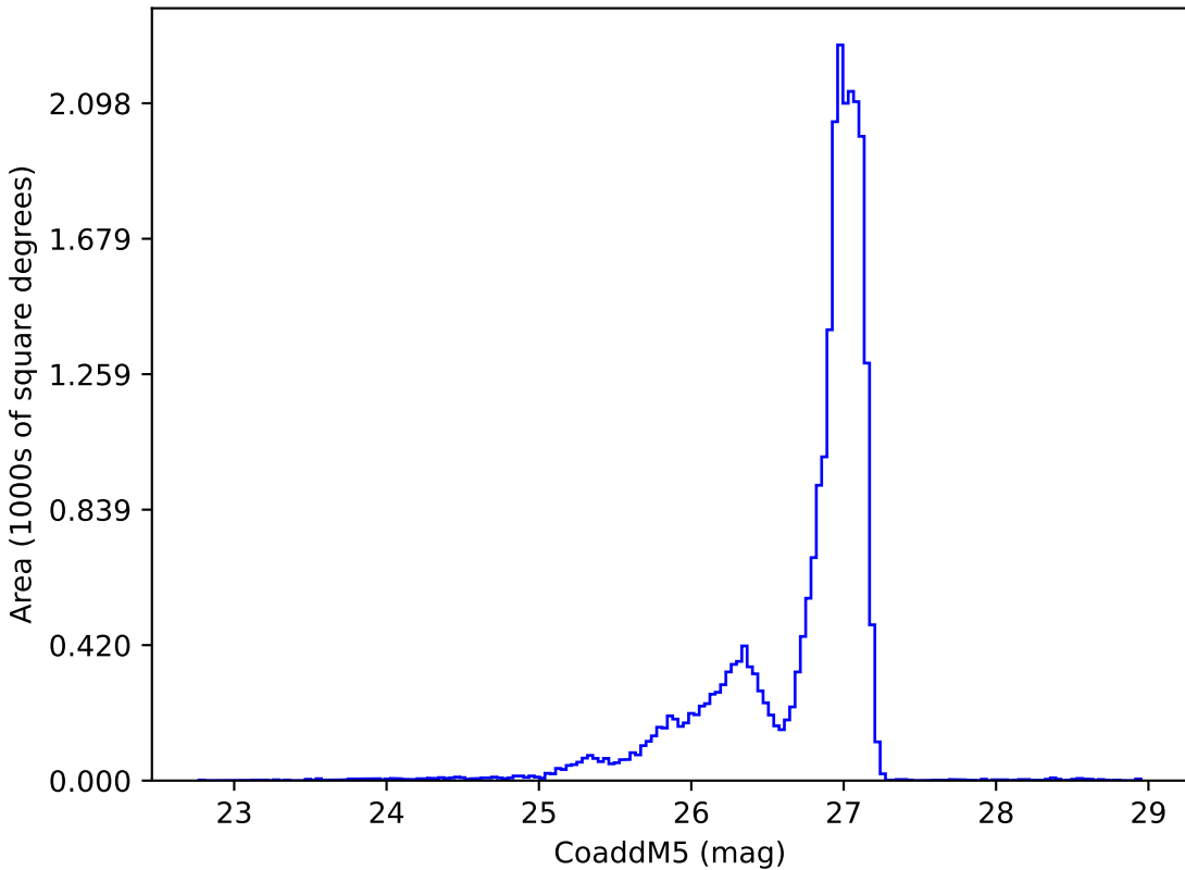
too_elab_r8_d2_ugrizy_v3.4_10yrs r: CoaddM5
