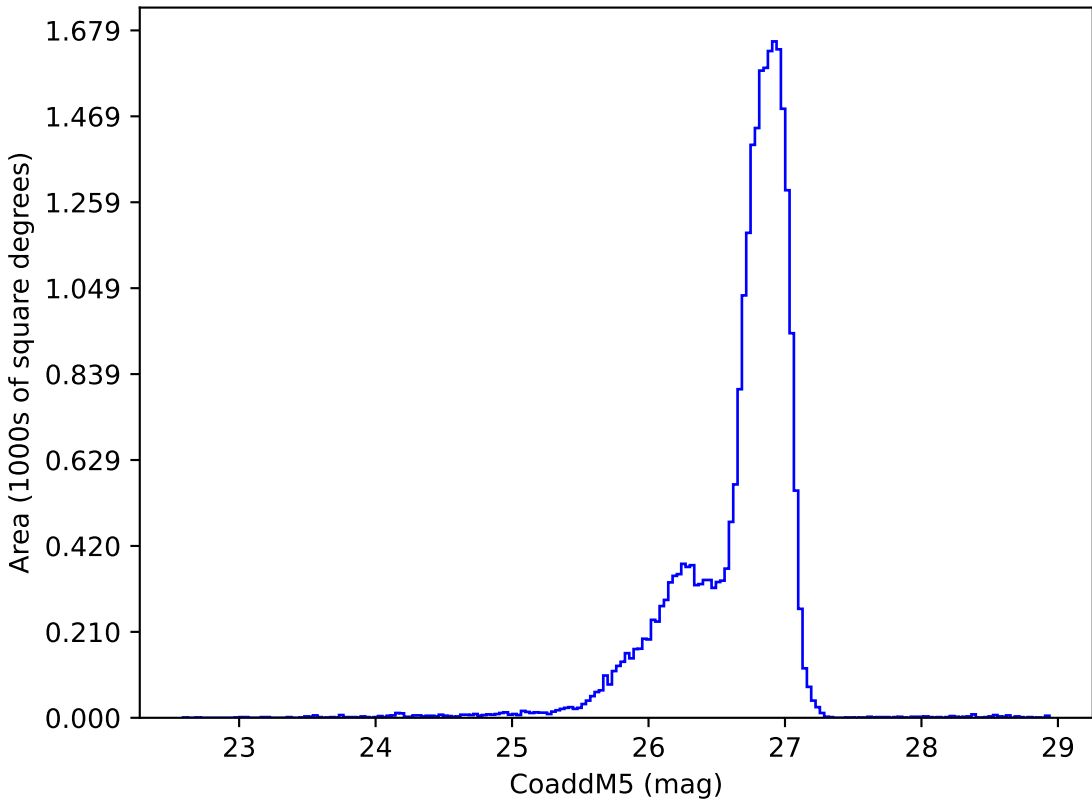
too_elab_r8_d2_ugrizy_v3.4_10yrs g: CoaddM5
