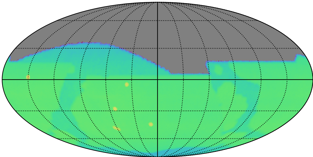
too_elab_r8_d2_ugrizy_v3.4_10yrs : CoaddM5
