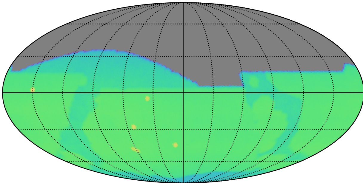
too_elab_r8_d2_ugrizy_v3.4_10yrs : CoaddM5
