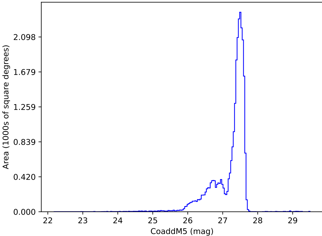
too_elab_r8_d2_ugrizy_v3.4_10yrs : CoaddM5
