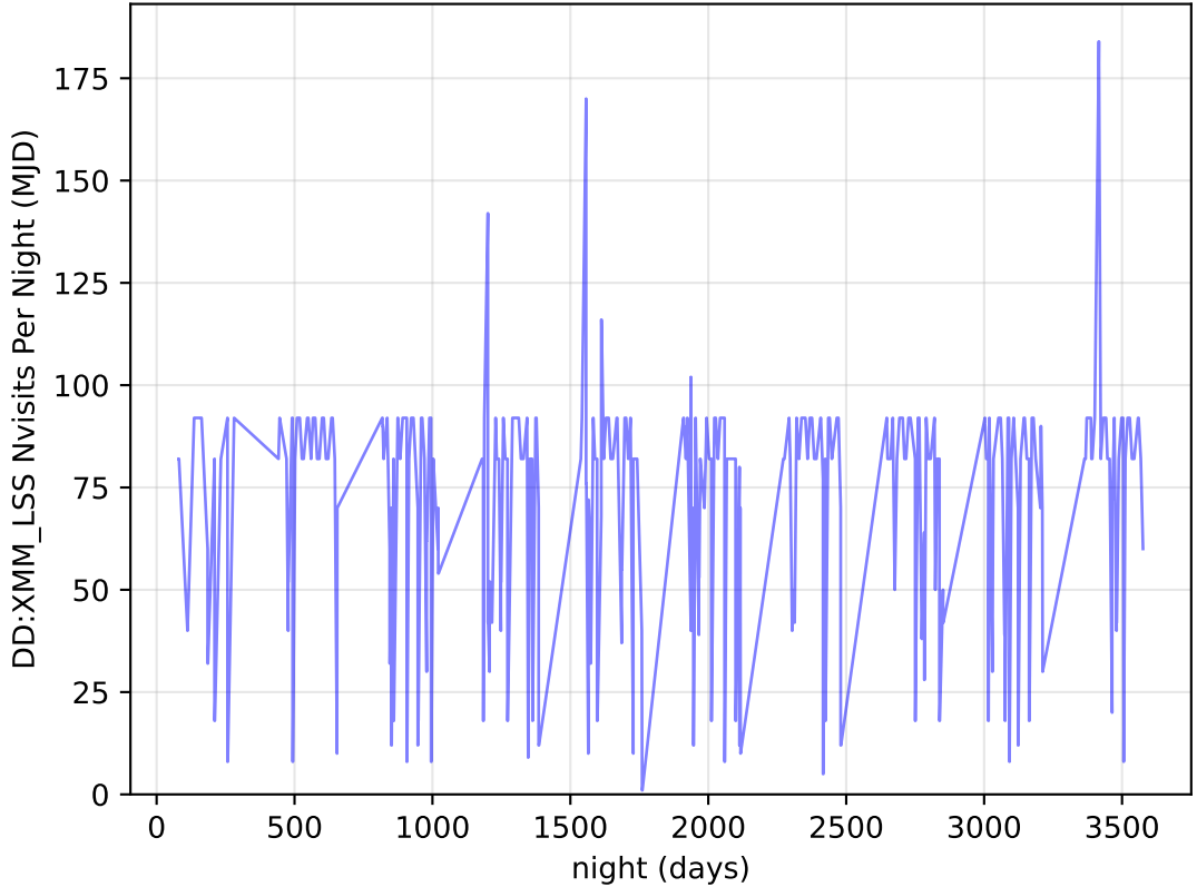
too_elab_r8_d2_ugrizy_v3.4_10yrs all bands: DD:XMM_LSS Nvisits Per Night
