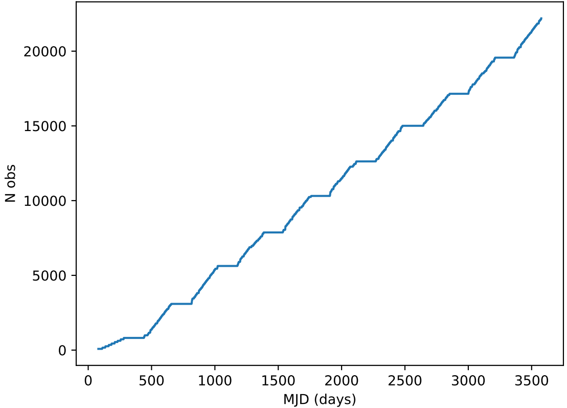
too_elab_r8_d2_ugrizy_v3.4_10yrs all bands: DD:XMM_LSS Cumulative NVisits
