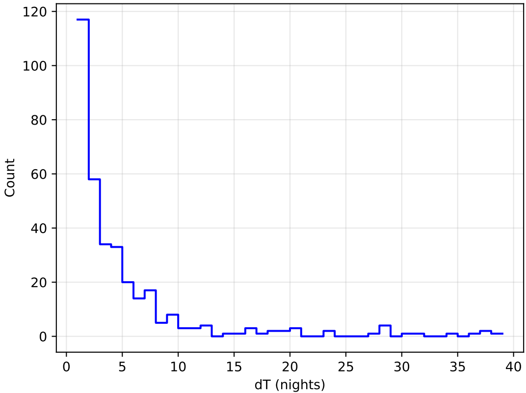
too_elab_r8_d2_ugrizy_v3.4_10yrs all bands: DD:WFD Delta Nights Histogram
