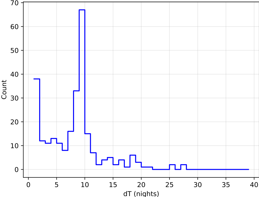
too_elab_r8_d2_ugrizy_v3.4_10yrs all bands: DD:ELAISS1 Delta Nights Histogram
