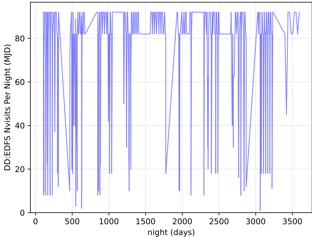
too_elab_r8_d2_ugrizy_v3.4_10yrs all bands: DD:EDFS Nvisits Per Night
