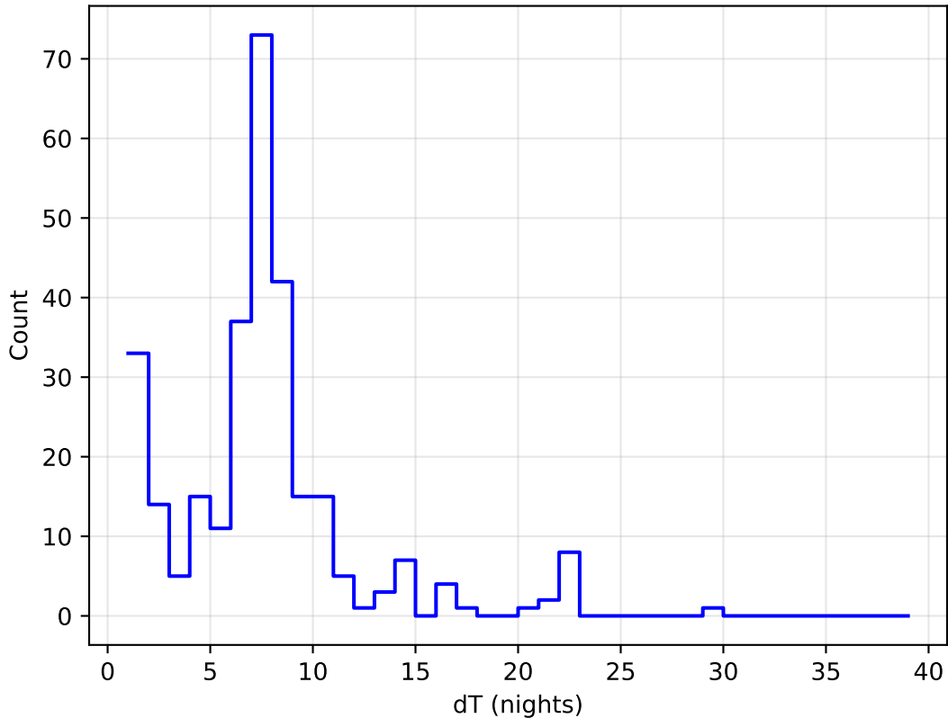
too_elab_r8_d2_ugrizy_v3.4_10yrs all bands: DD:EDFS Delta Nights Histogram
