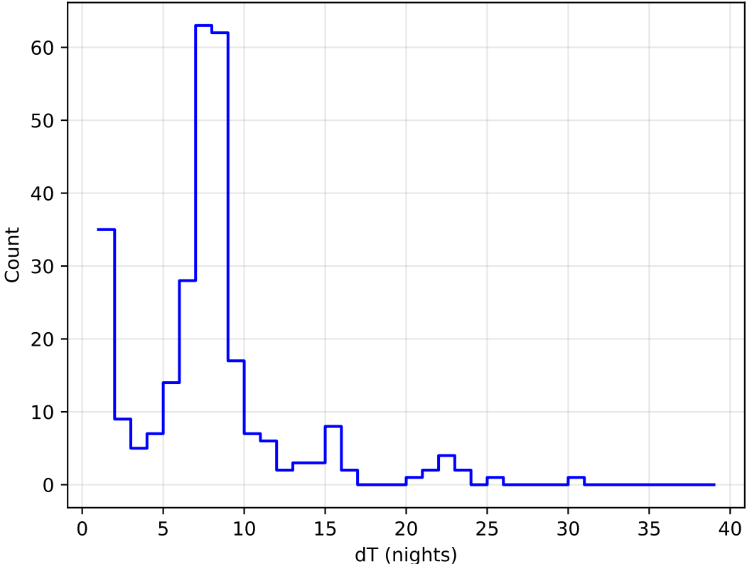
too_elab_r8_d2_ugrizy_v3.4_10yrs all bands: DD:ECDFS Delta Nights Histogram
