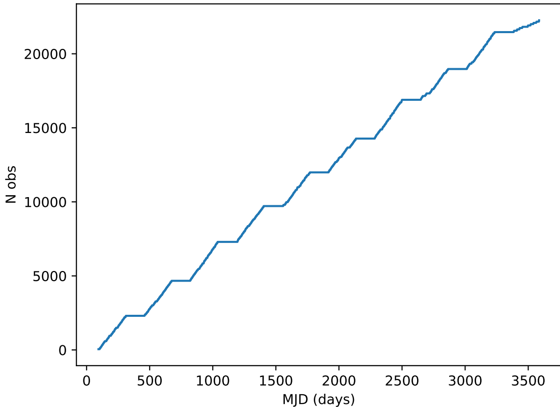
too_elab_r8_d2_ugrizy_v3.4_10yrs all bands: DD:ECDFS Cumulative NVisits
