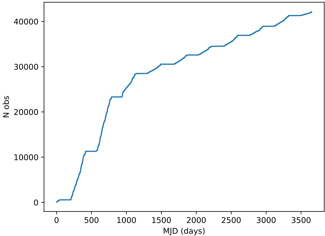
too_elab_r8_d2_ugrizy_v3.4_10yrs all bands: DD: COSMOS Cumulative NVisits
