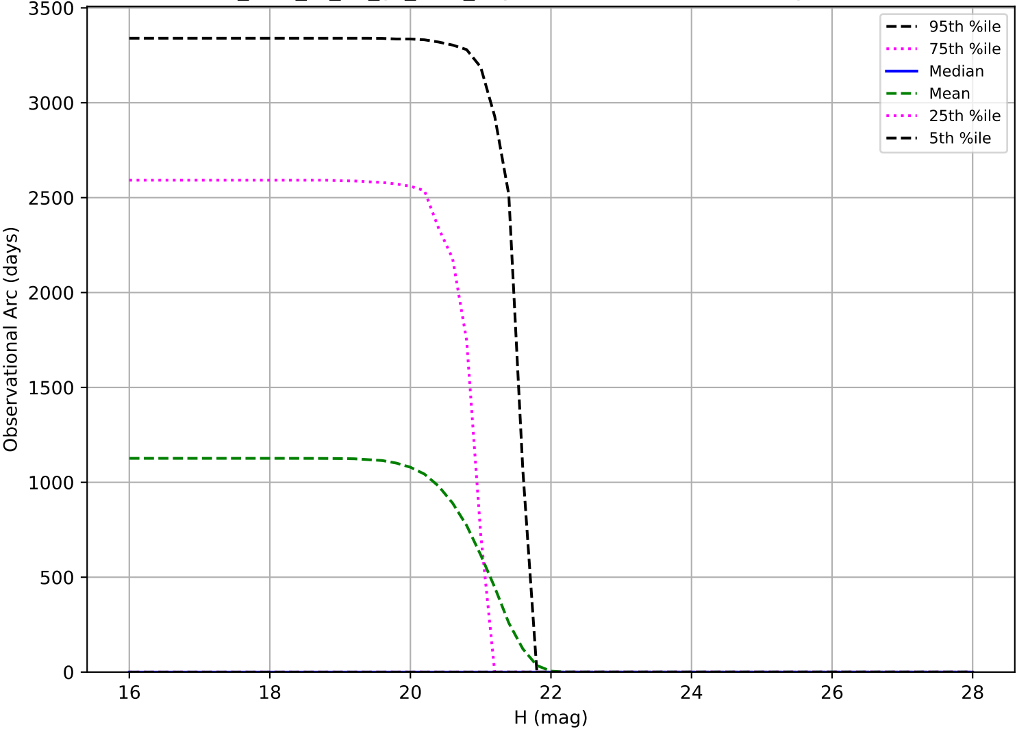
too_elab_r8_d2_gz_v3.4_10yrs: Observational Arc Length Vatra
