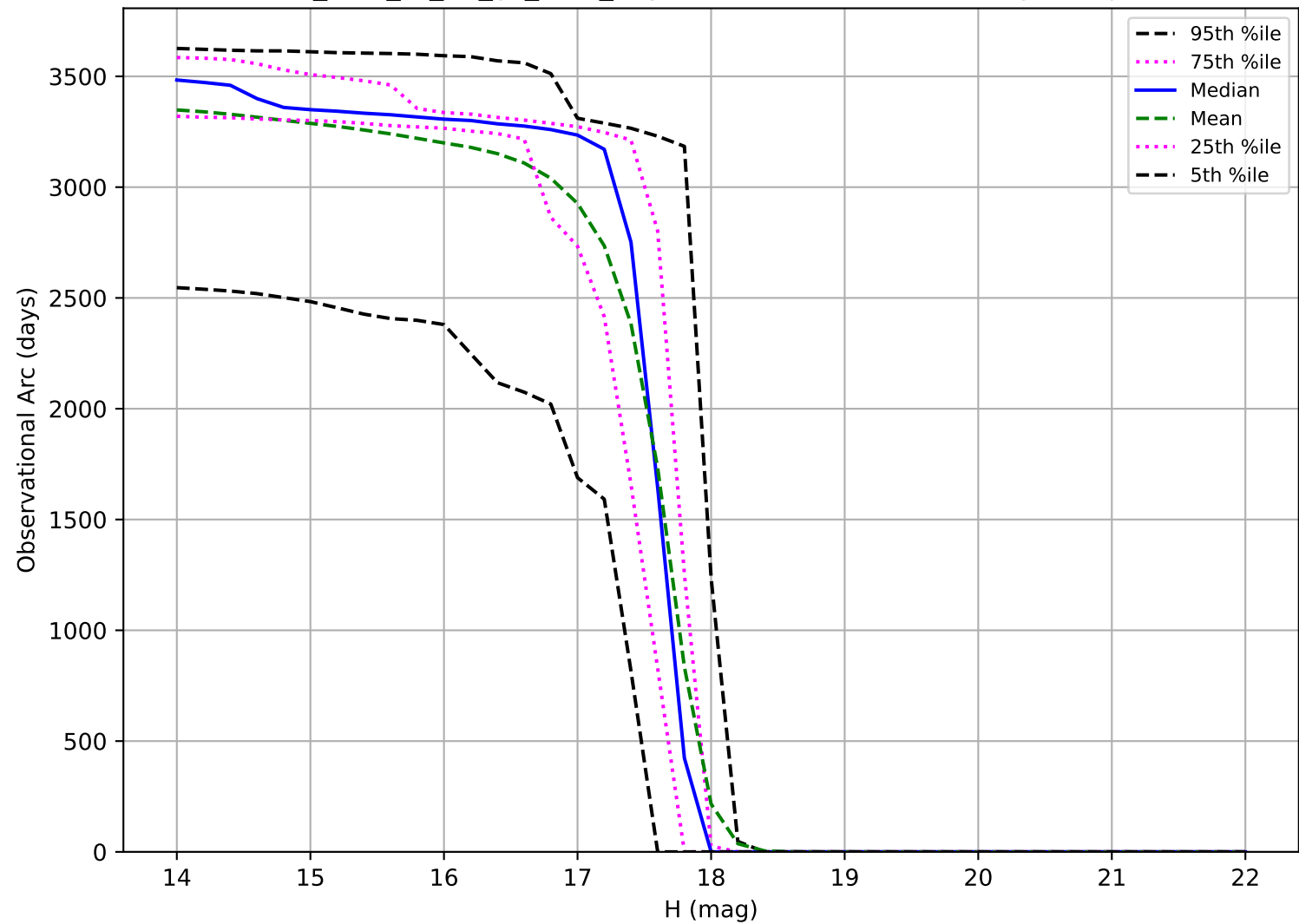
too_elab_r8_d2_gz_v3.4_10yrs: Observational Arc Length Trojan
