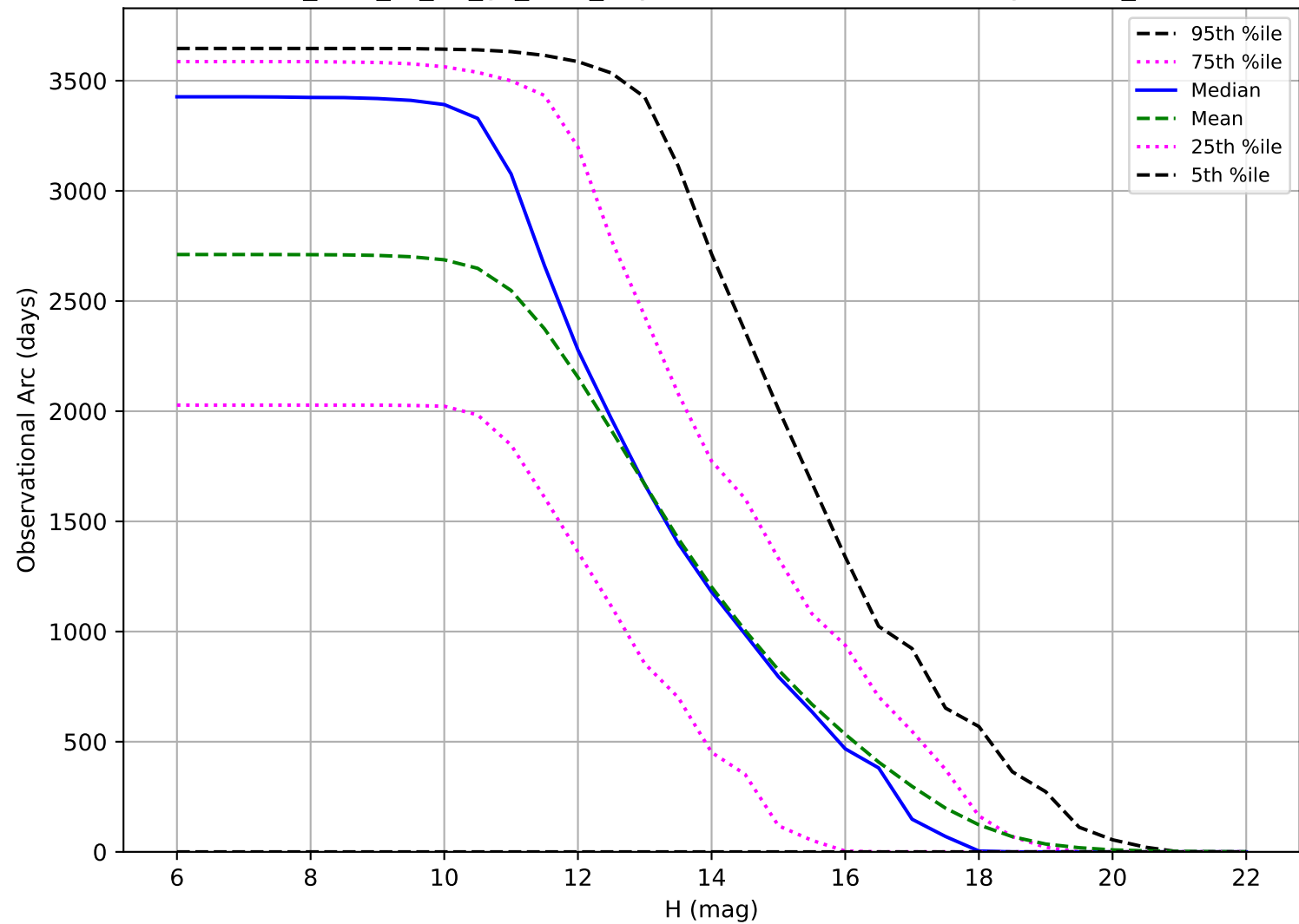
too_elab_r8_d2_gz_v3.4_10yrs: Observational Arc Length OCC_r5
