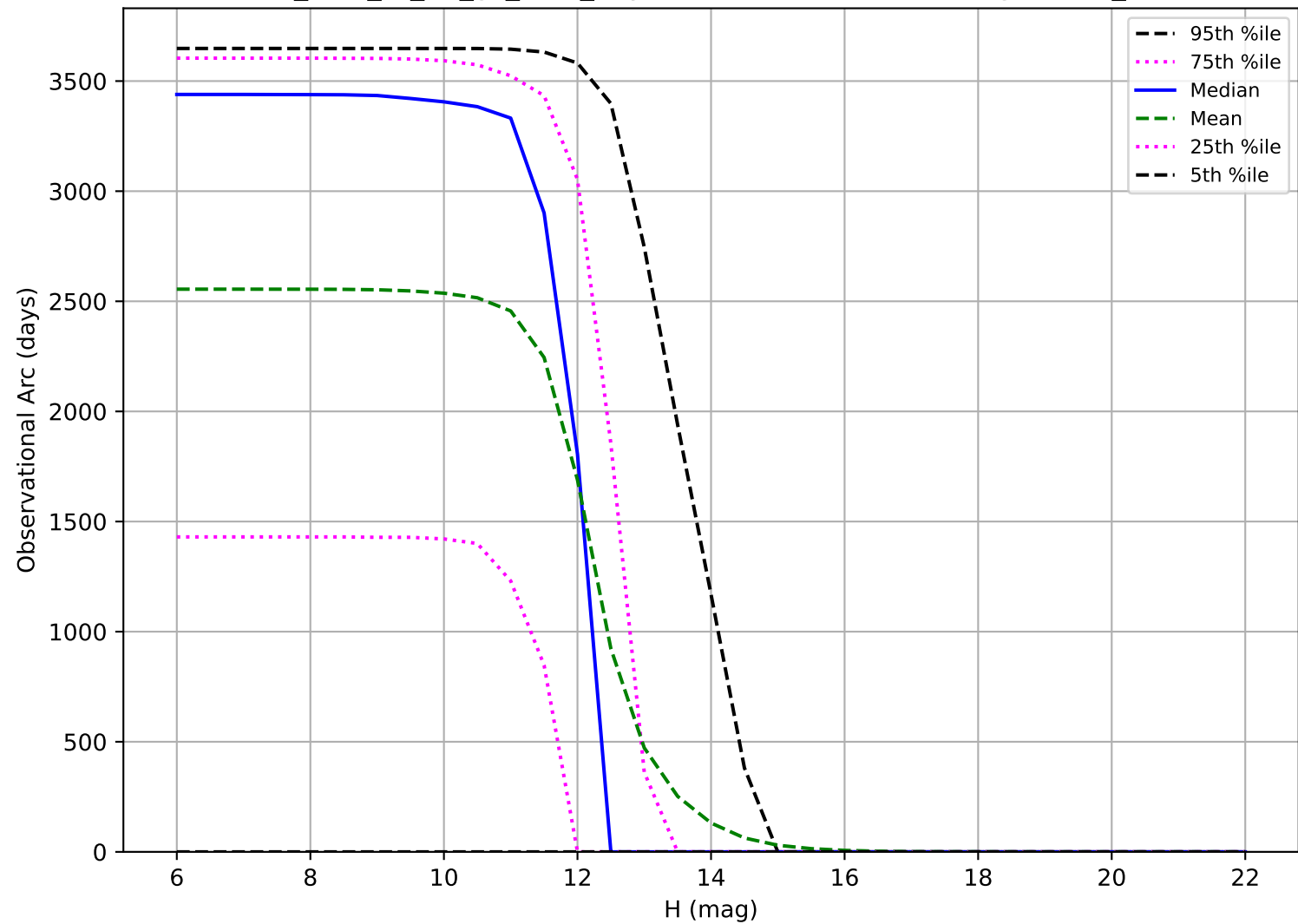
too_elab_r8_d2_gz_v3.4_10yrs: Observational Arc Length OCC_r20
