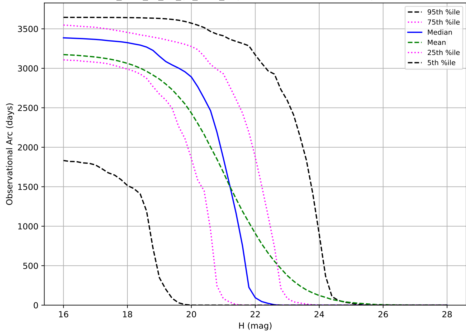
too_elab_r8_d2_gz_v3.4_10yrs: Observational Arc Length NEO
