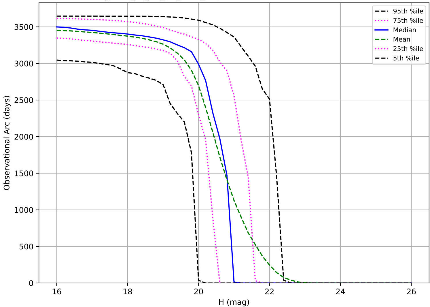
too_elab_r8_d2_gz_v3.4_10yrs: Observational Arc Length MBA
