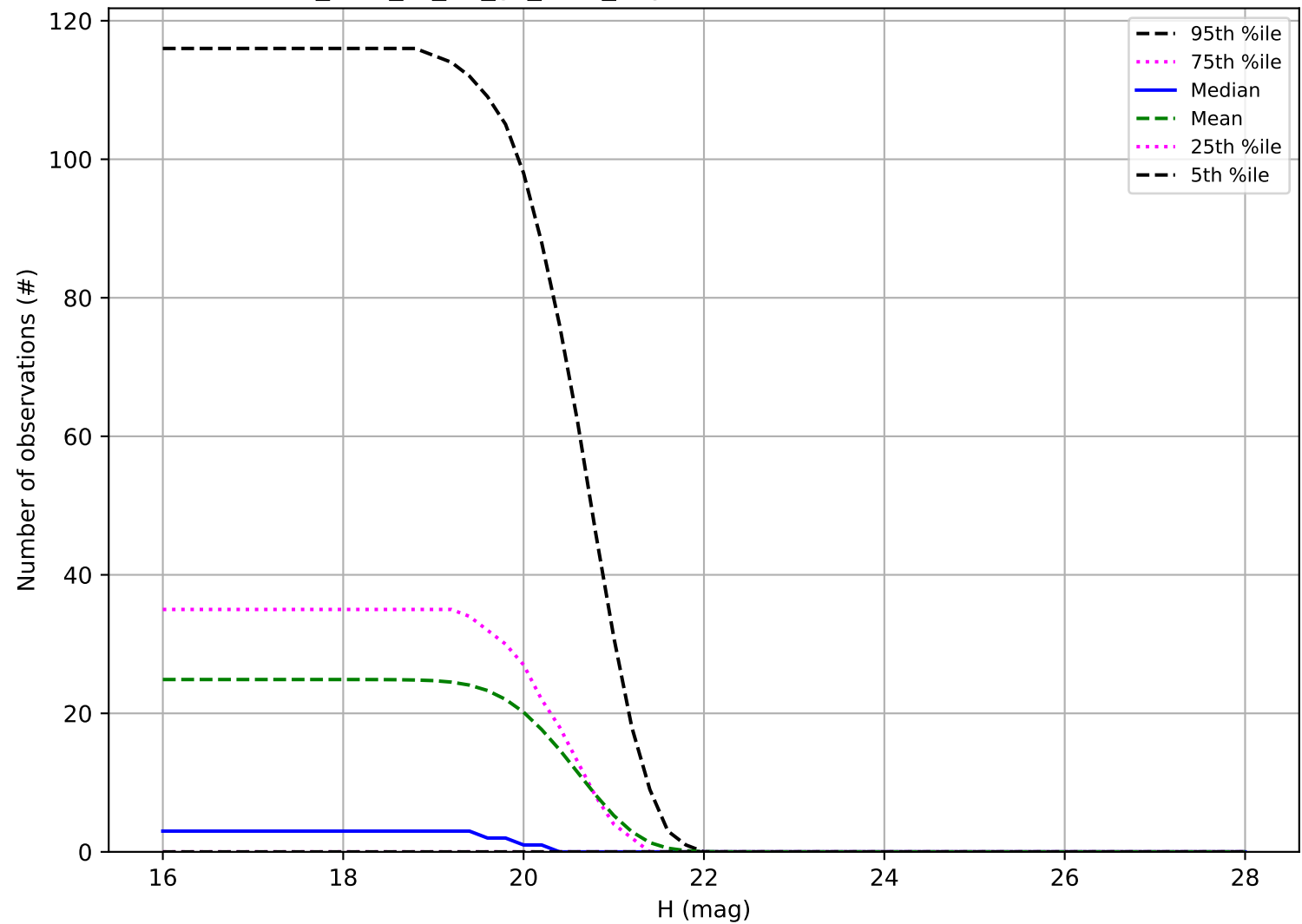
too_elab_r8_d2_gz_v3.4_10yrs: Number of observations Vatira
