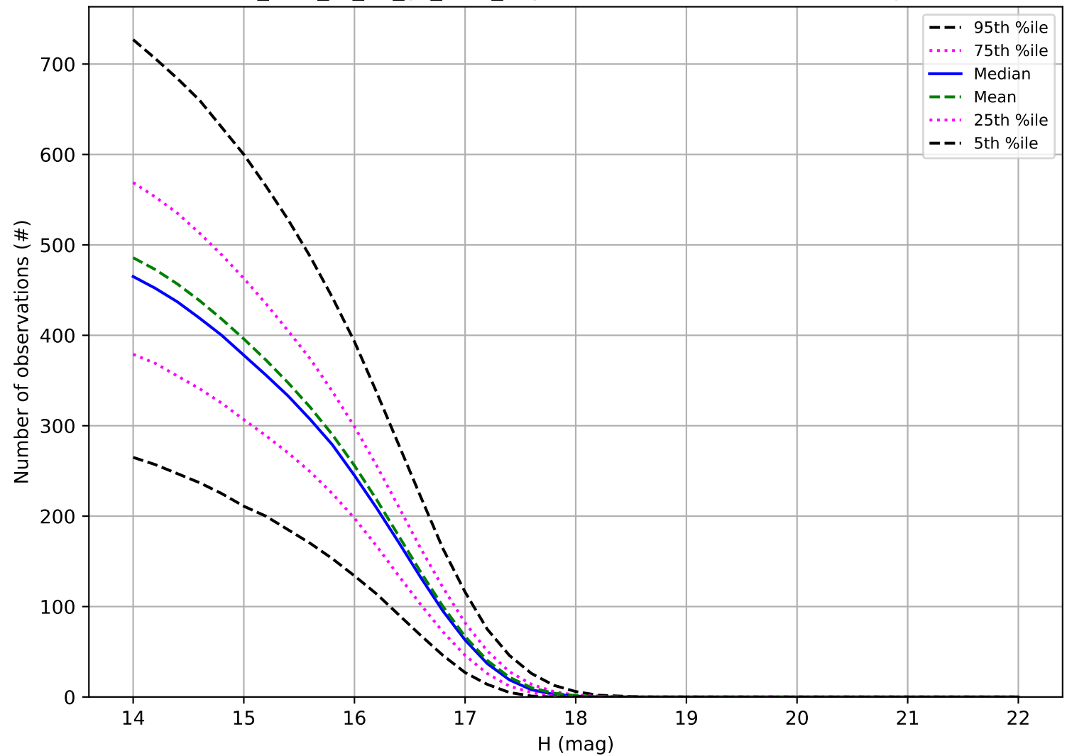
too_elab_r8_d2_gz_v3.4_10yrs: Number of observations Trojan
