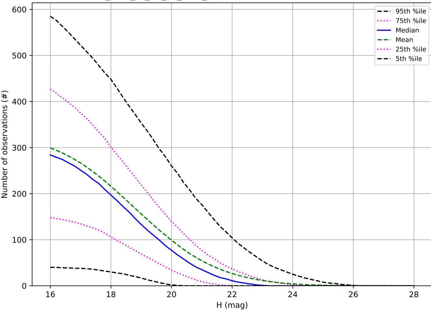
too_elab_r8_d2_gz_v3.4_10yrs: Number of observations PHA
