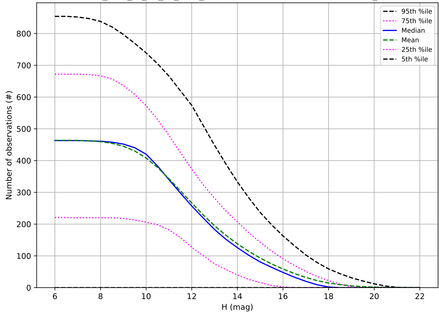
too_elab_r8_d2_gz_v3.4_10yrs: Number of observations OCC_r5
