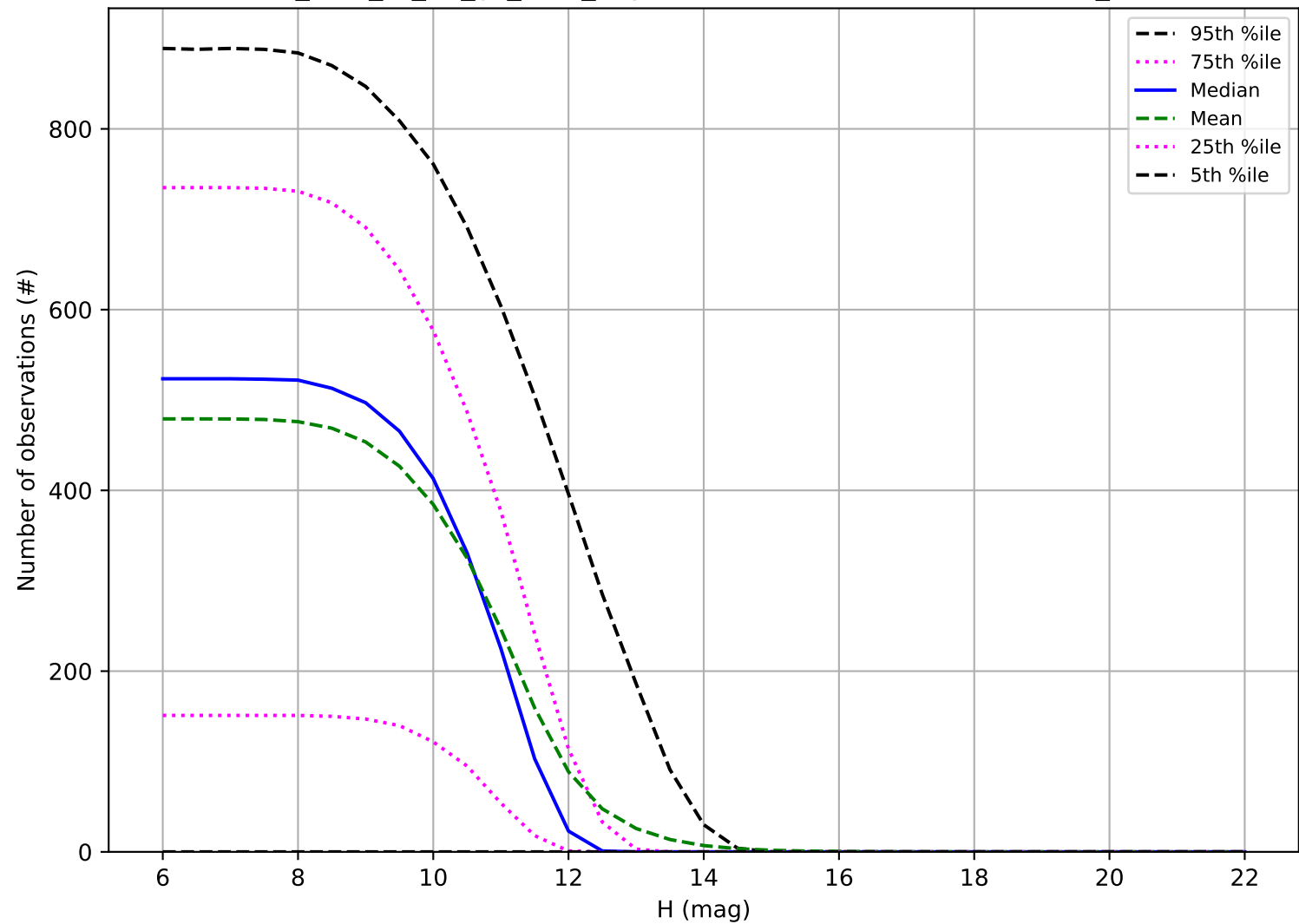
too_elab_r8_d2_gz_v3.4_10yrs: Number of observations OCC_r20
