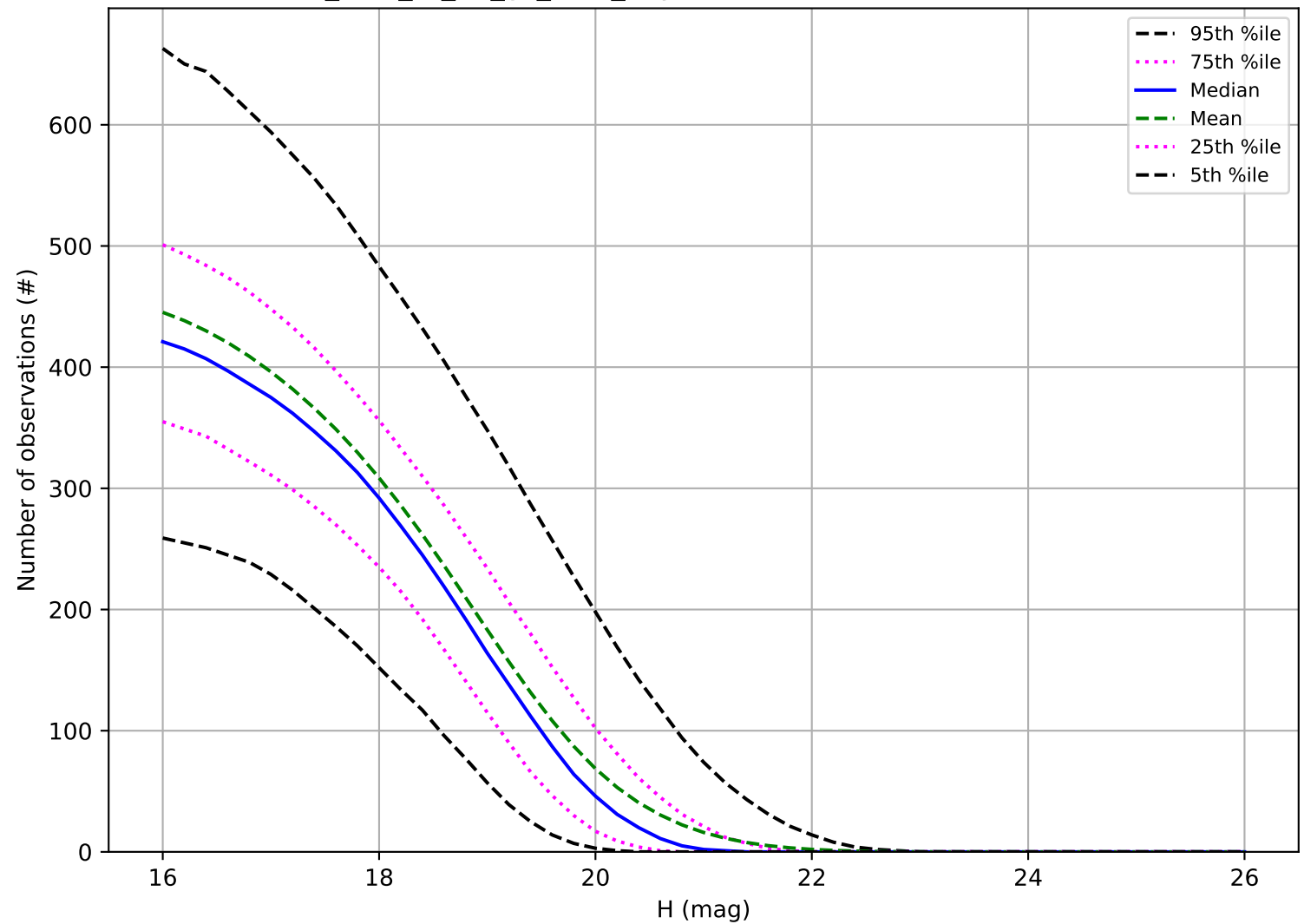
too_elab_r8_d2_gz_v3.4_10yrs: Number of observations MBA
