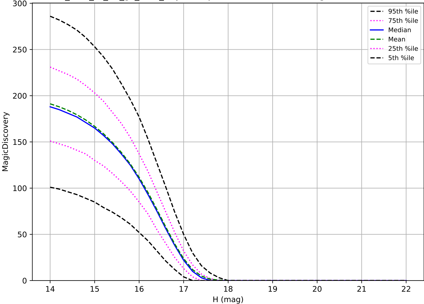
too_elab_r8_d2_gz_v3.4_10yrs: Trojan 6 detections in 60 nights detection loss
